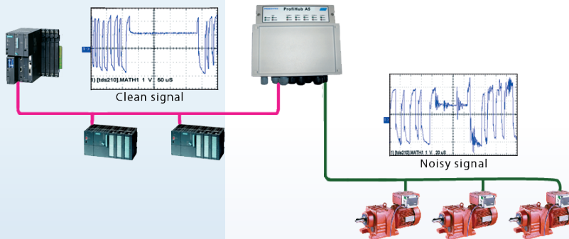
Example of the barrier function of the ProfiHub. Noise and EMC disturbances will not affect the backbone or the other channels
